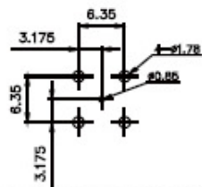
RECOMMENDED PC BOARD LAYOUT WITHOUT MOUNTING POSTS
