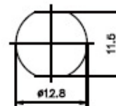
RECOMMENDED MOUNTING HOLE MAXIMUM PANEL THICKNESS: 6.5MM
